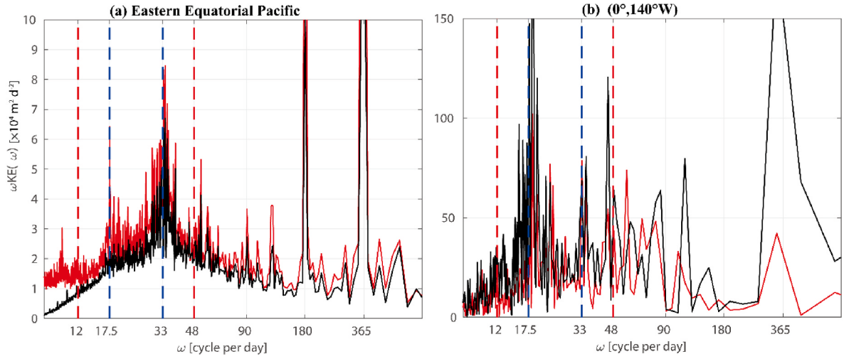
Fig. 1. The frequency spectra (lines) of (a) the surface KE averaged over the eastern equatorial Pacific based on AVISO (black line) and HYCOM (red line) and (b) the KE at (0^\circ, 140^\circ\text{W}) and the depth of 10 m based on TAO (black line) and HYCOM (red line). The spectra are plotted in variance-preserving form (i.e., spectrum KE ( \omega ) multiplied by frequency \omega ). The dashed lines denote the periods of 12, 17.5, 33, and 48 days from left to right respectively. The range of the ordinate is limited to 0 - 10 \times 10^4 \text{ m}^2 \text{d}^{-3} in (a) and 0 - 150 \times 10^4 \text{ m}^2 \text{d}^{-3} in (b) to highlight the high-frequency spectra.
